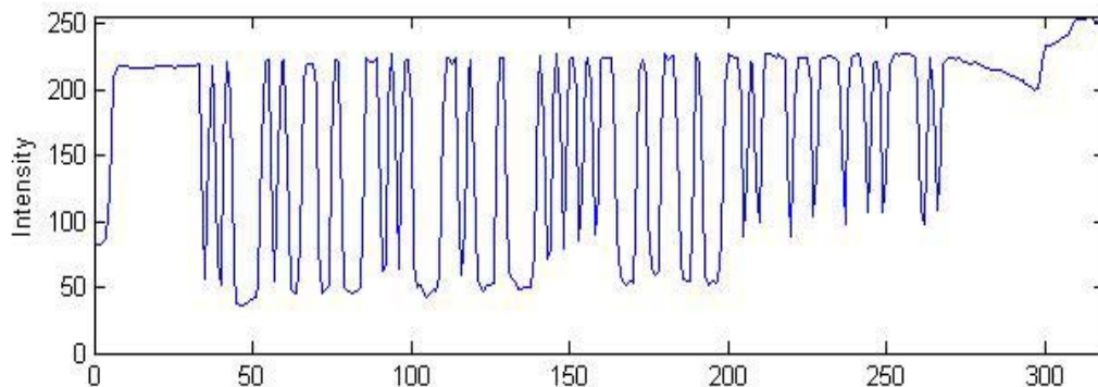
Figure 9: A sample row across the barcode image.
